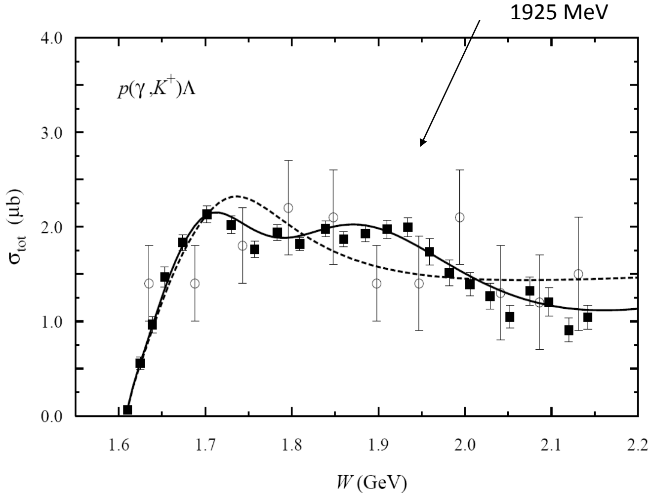
FIG. 1. Total cross section for K^+ \Lambda photoproduction on the proton. The dashed line shows the model without the D_{13}(160) resonance, while the solid line is obtained by including the D_{13}(160) state. The new SAPHIR data [6] are denoted by the solid squares, old data [22] are shown by the open circles.
